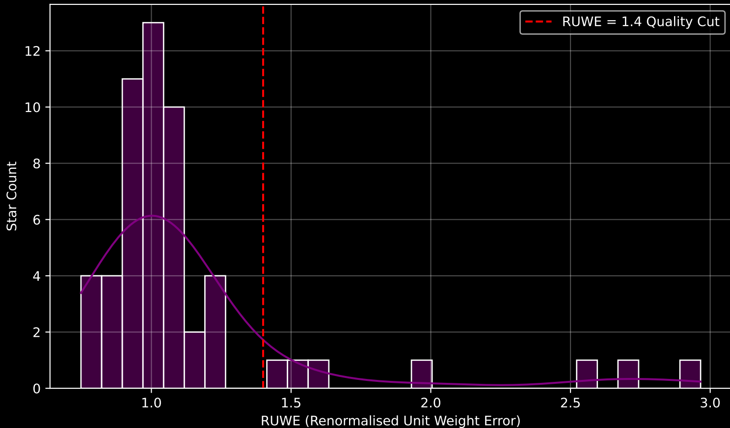
GAPOGEE DR17 Field [282-32-O] RUWE Distribution (n= 55)
