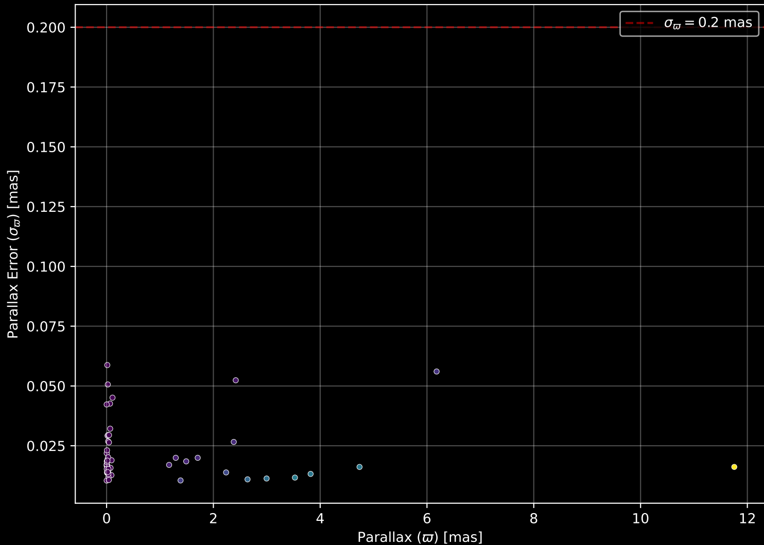
APOGEE DR17 Field: [282-32-O] Parallax Quality (n= 55)
