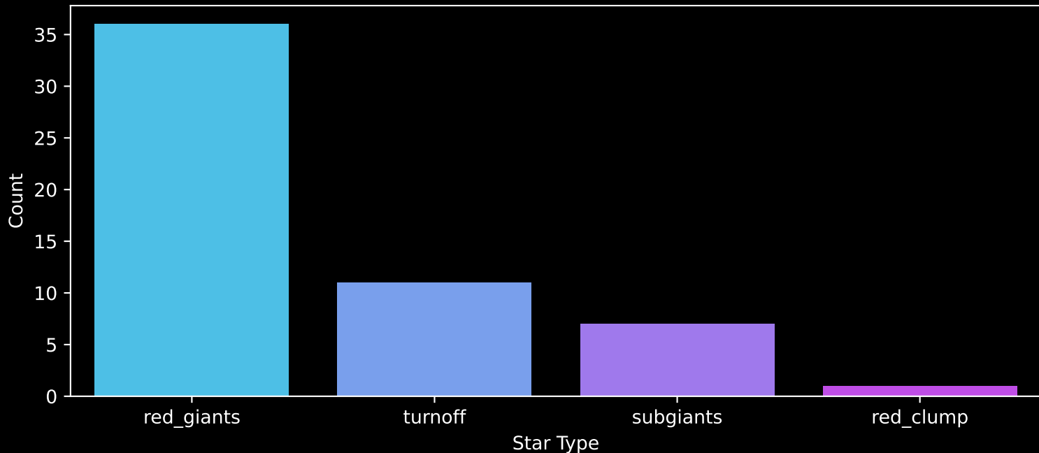
APOGEE DR17 Field: [282-32-O] Count plot of Star Type
