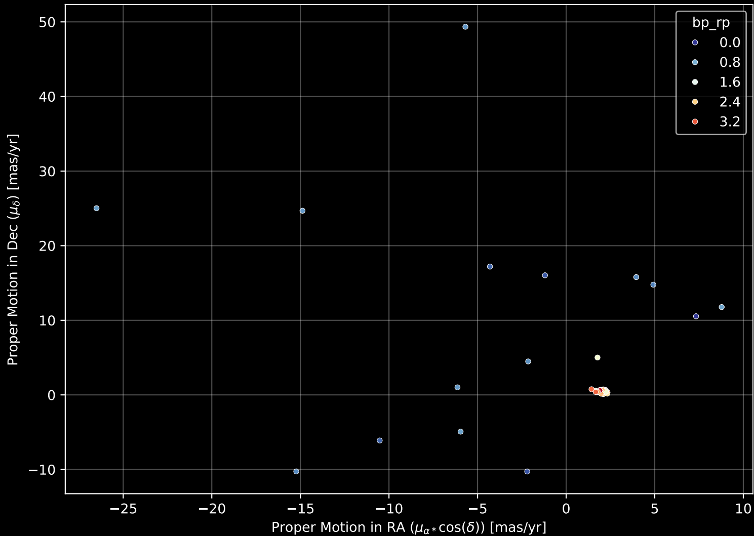
APOGEE DR17 Field: [282-32-O] Proper Motion Diagram (n= 55)
